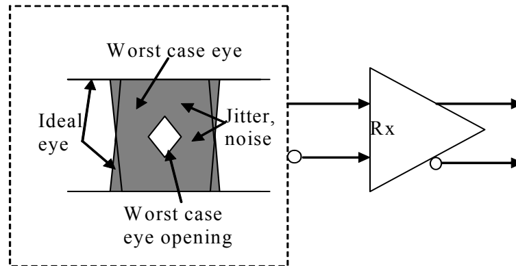
Figure 7. Worst case eye/jitter signaling condition for receiver tolerance testing.
