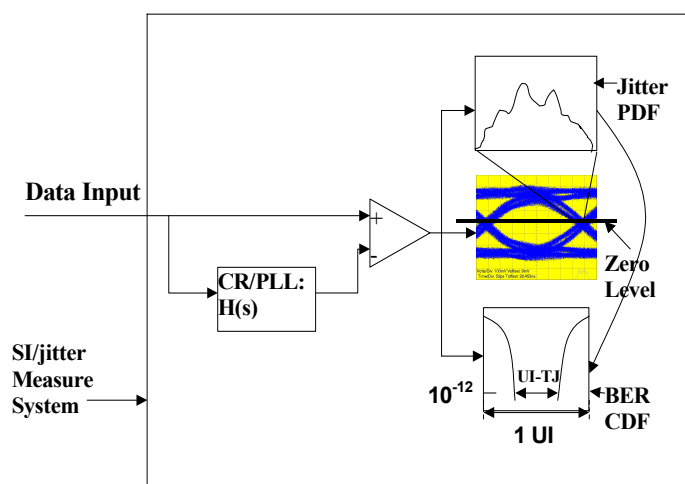
Figure 2. A schematic diagram shows the correct setup for JNB output testing.
