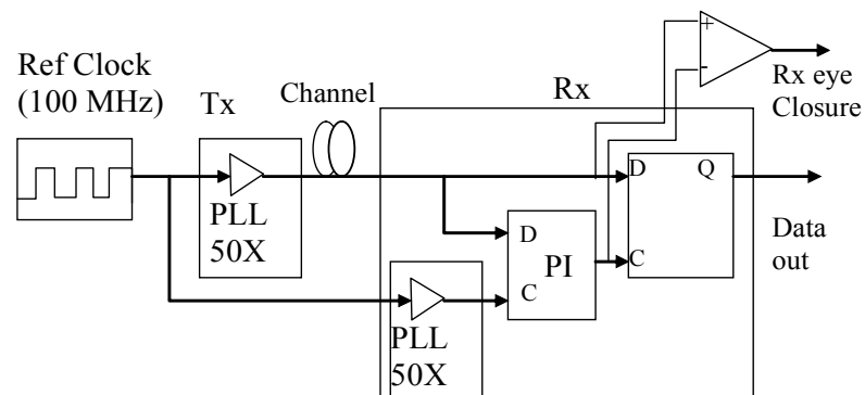
Figure 1. PCIe II link architecture diagram using a phase interpolator (PI) or an over-sampling (OS) in its receiver.
