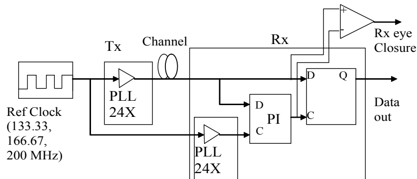
Figure 9. FB DIMM link architecture block diagram.
